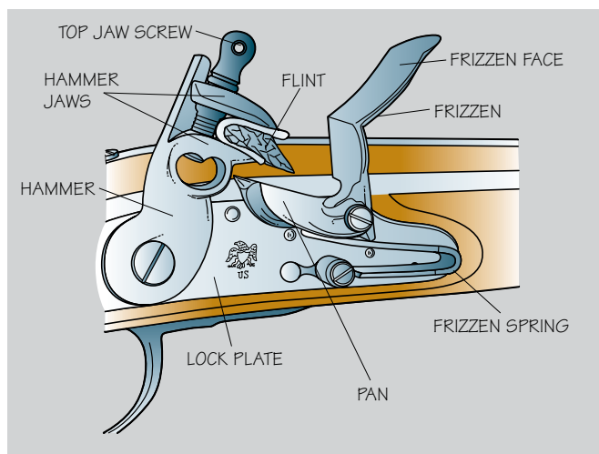
Flintlock action
