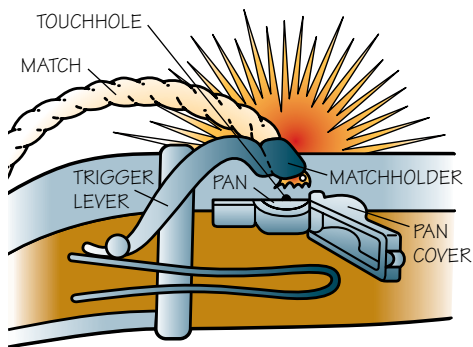
Matchlock action
