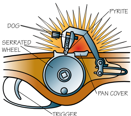
Wheel lock action
