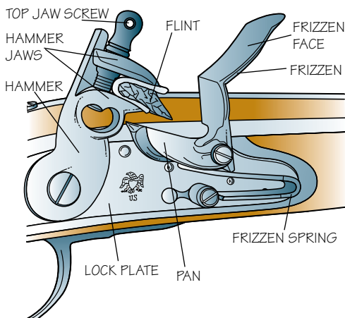
Flintlock action
